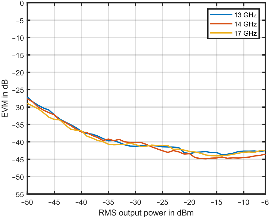
Measured EVM of a 4 GHz OFDM signal, full allocation, SCS: 960 kHz, modulation: QPSK, optimize EVM turned on, using the FSW signal and spectrum analyzer with the R&S®FSW-K575 I/Q noise cancellation option (IQNC with 50 iterations)
