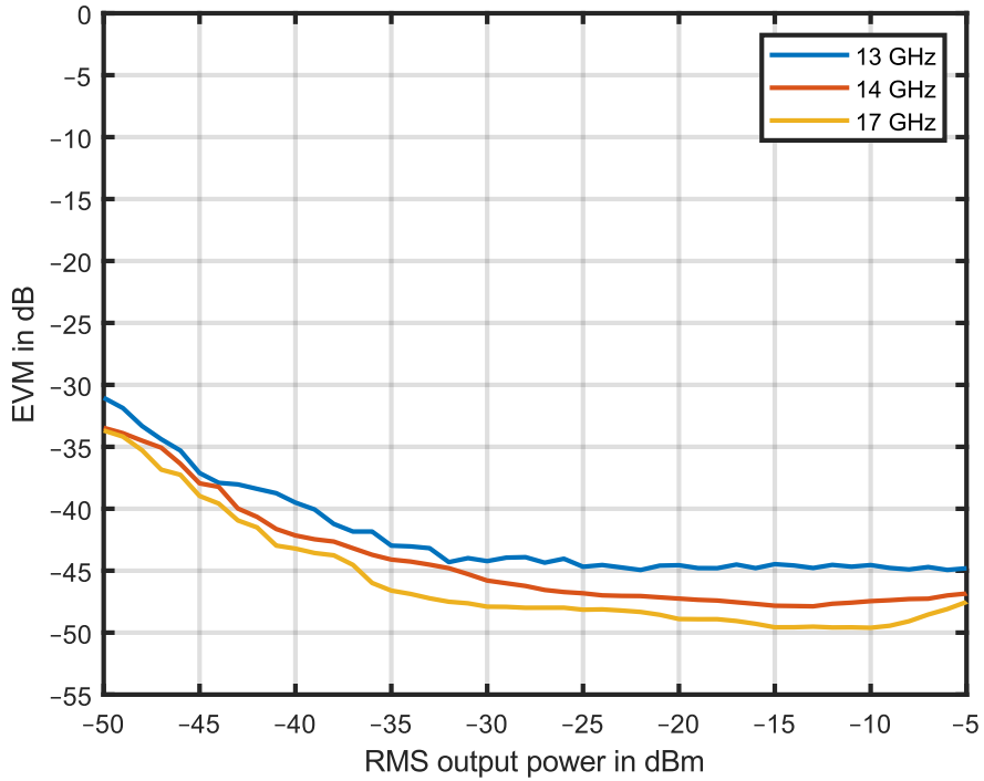
Measured EVM of a 2 GHz 5G NR signal, full allocation, SCS: 960 kHz, modulation: 256QAM, optimize EVM turned on, using the FSW signal and spectrum analyzer with the R&S®FSW-K575 I/Q noise cancellation option (IQNC with 50 iterations)
