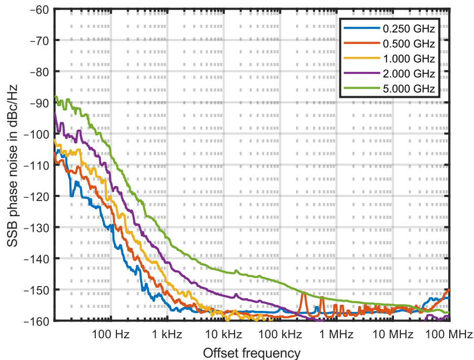
Measured SSB phase noise for a sine wave, unused output terminated by 50 \Omega , bias = 0 V, output voltage = 0.5 V
