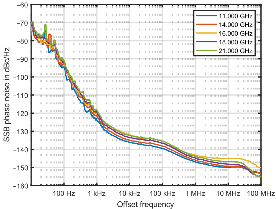
Measured SSB phase noise, CW mode, RF output
