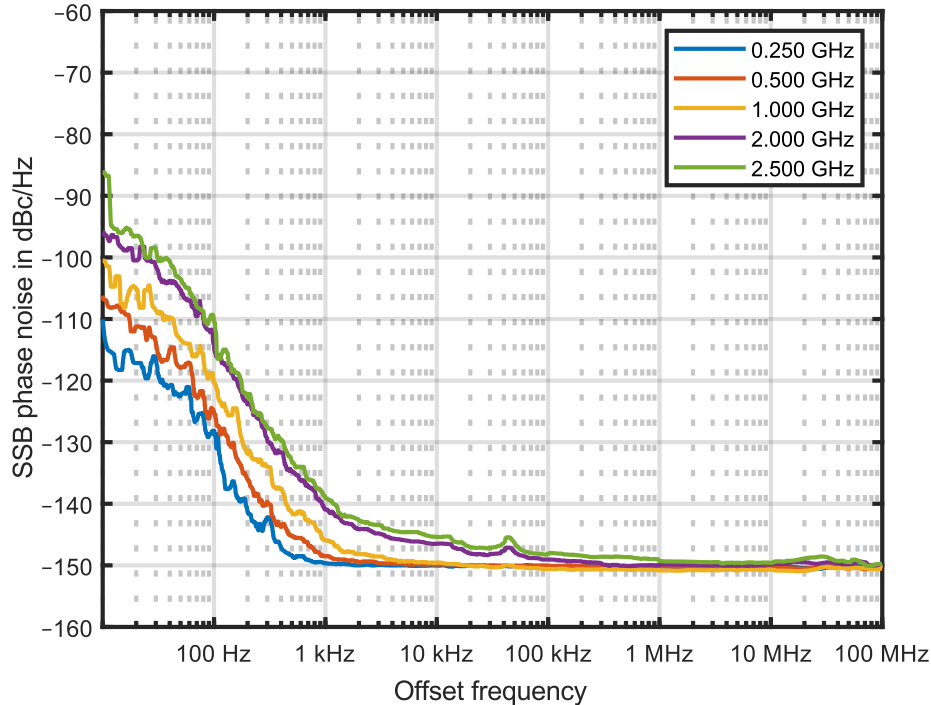
Measured SSB phase noise for a sine wave, unused output terminated by 50 \Omega , bias = 0 V
