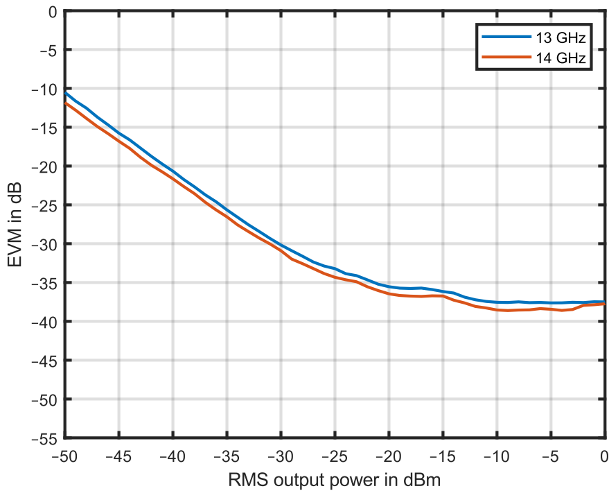
Measured EVM of a 4.32 GHz IEEE 802.11ay EDMG signal, NCB2, modulation: 16QAM, optimize EVM turned on, using the FSW signal and spectrum analyzer
